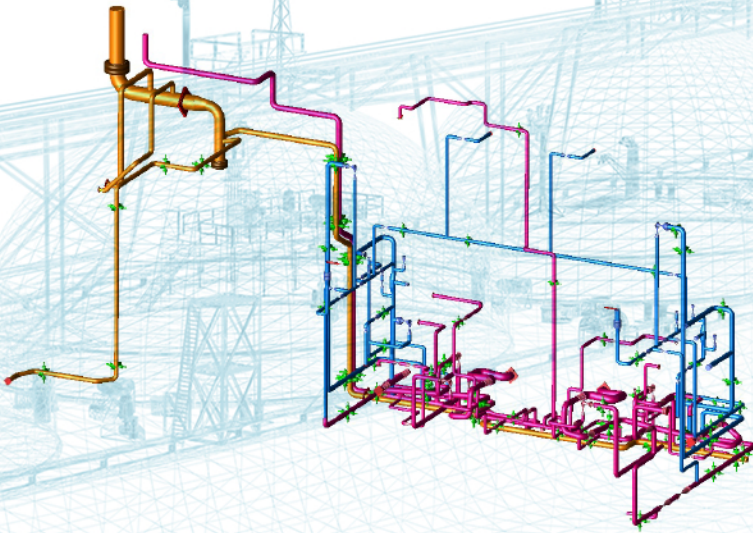
Subsea Manifold (Fast Track)
