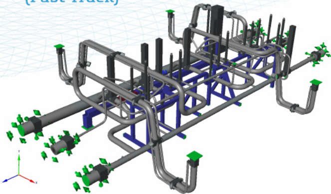
Subsea Manifold (Fast Track)
